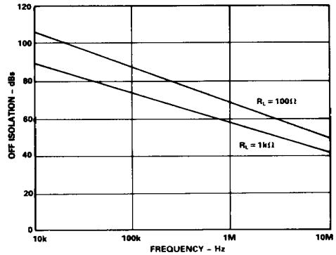
Off Isolation vs. Signal Frequency; Dual or Single 15V Supplies, T_A = +25^\circ\text{C}
