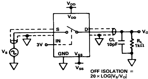
TEST CIRCUIT 5 OFF ISOLATION
