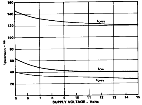
Switching Time vs. Supply Voltage (Single Supply): T_A = +25^\circ\text{C} . (Note: See Test Circuit 4. For V_{DD} < 10\text{V} , V_S = V_{DD} )
