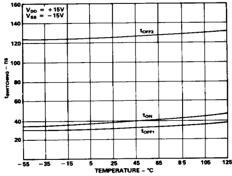
Switching Time vs. Temperature: Dual Supply Voltage
