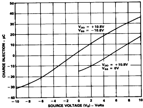
Charge Injection vs. Source Voltage ( V_S ) for Dual and Single 10.8V Supplies: T_A = +25^\circ\text{C}
