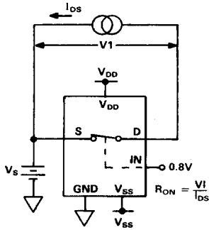
TEST CIRCUIT 1 R_{ON}
