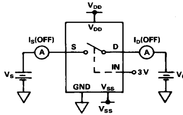
TEST CIRCUIT 2 I_S(\text{OFF}), I_D(\text{OFF})
