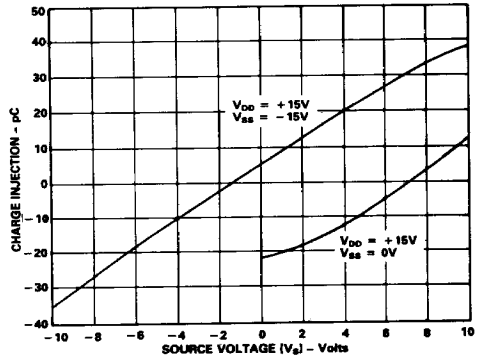
Charge Injection vs. Source Voltage ( V_S ) for Dual and Single 15V Supplies: T_A = +25^\circ\text{C}
