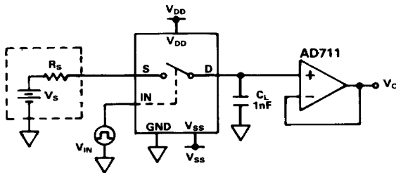
TEST CIRCUIT 7 CHARGE INJECTION
