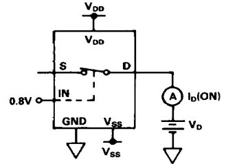
TEST CIRCUIT 3 I_D(\text{ON})
