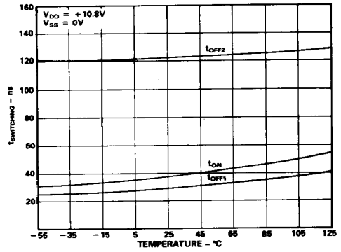
Switching Time vs. Temperature: Single Supply Voltage
